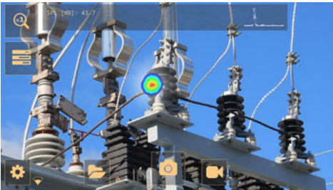
Partial Discharge
