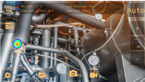
Compressed Air Leak
